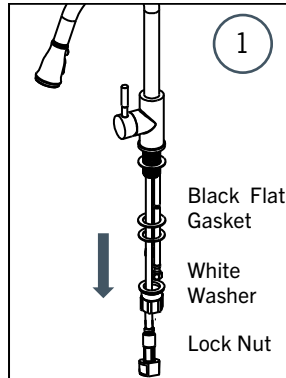
Faucet Assembly (C)
