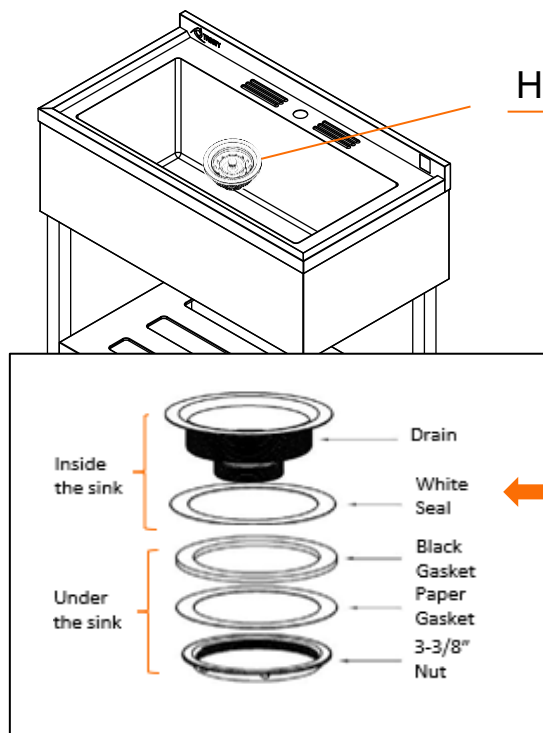
Drain Assembly (H)
