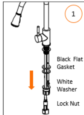
Faucet Assembly (F)
